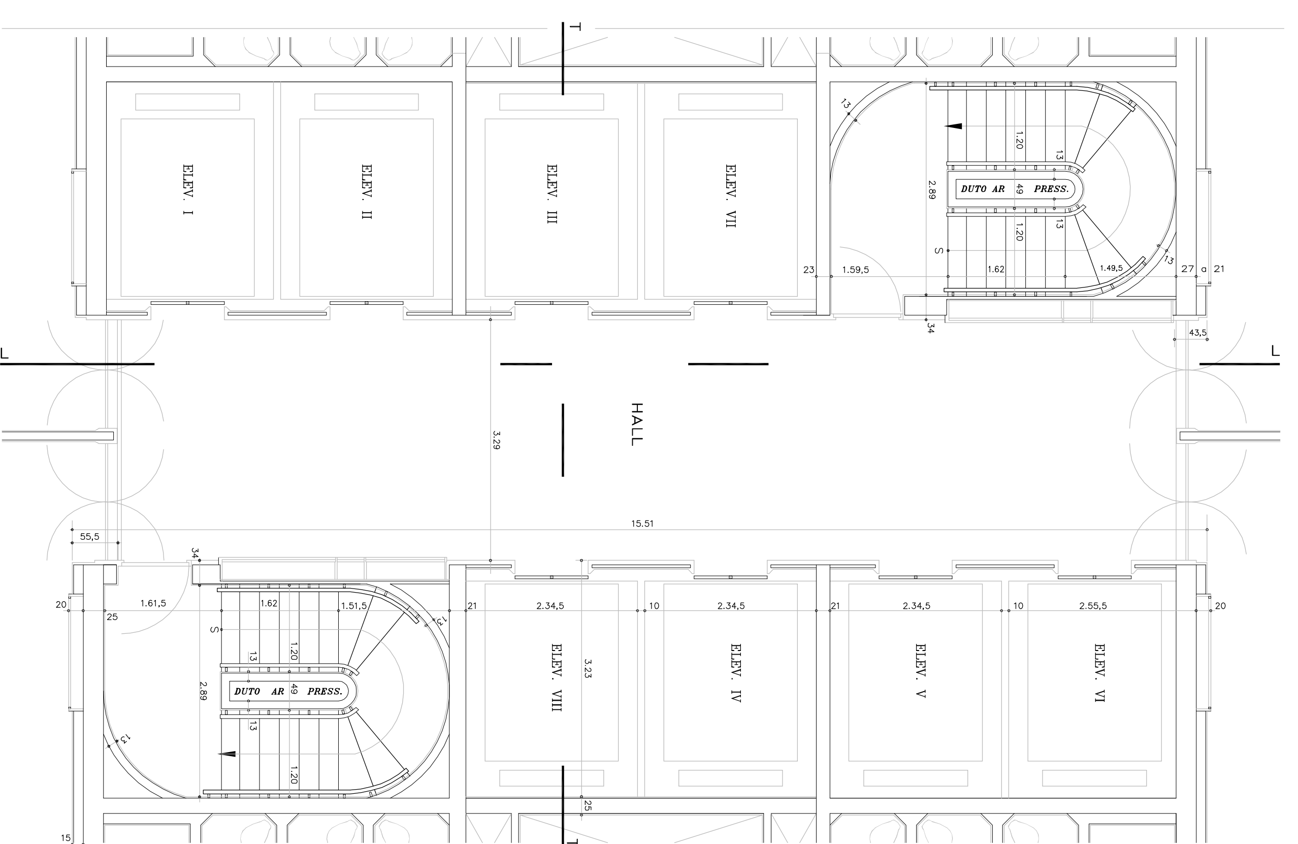
PLANTA DO HALL – ANDARES 1/3/5/7/9/11/13
